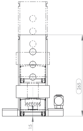
JHS 10 KU | Art.No. 01 020 105-O | Frontansicht | Front view
