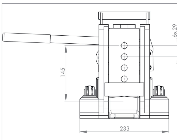
JH 6 G plus | Art.No. 01 060 102-G | Frontansicht | Front view
