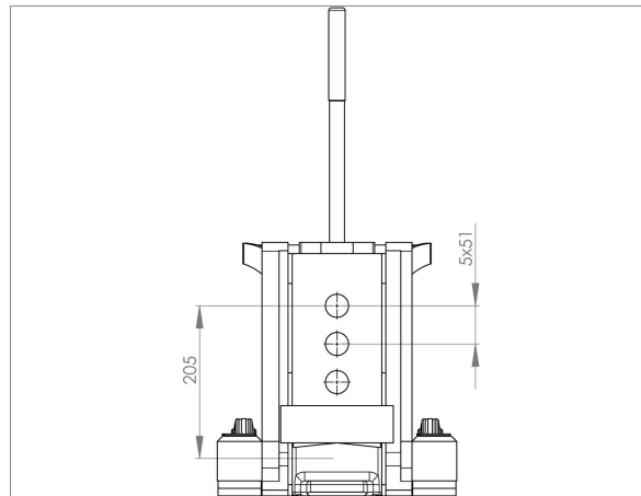
JH 20 G plus EX | Art-No. 11 620 106-G | Frontansicht | Front view
