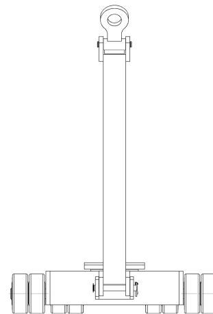
JLB 20 G | Art-No. 09 202 140-V | Frontansicht | Front view
