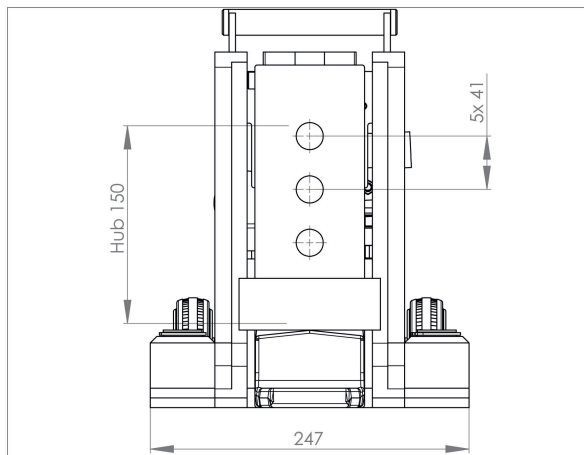
JH 10 G plus | Art.-No. 01 100 102-G | Frontansicht | Front view
