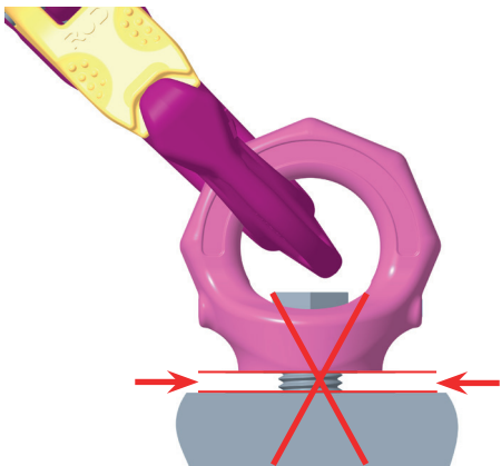
Abb./Pic./Image 4: The lifting point must be fully bolted in.
