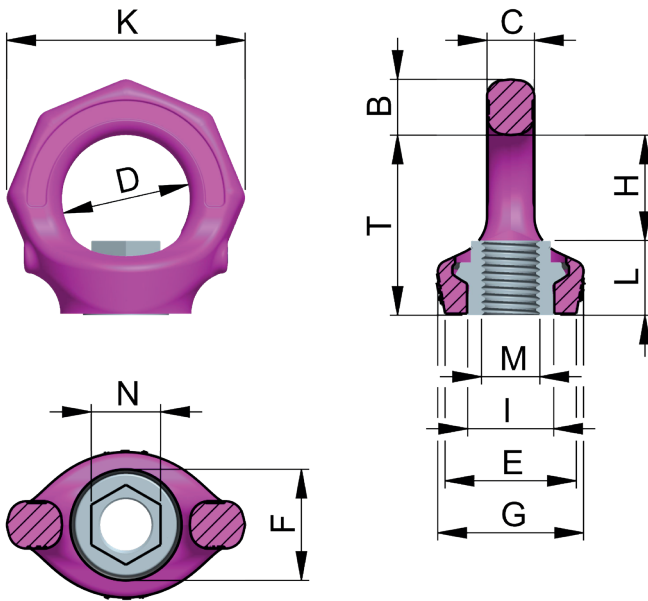
Pic. 5: Bemaßung
