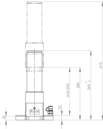
JHS 10 | Art.No. 01 020 101-O | Frontansicht | Front view
